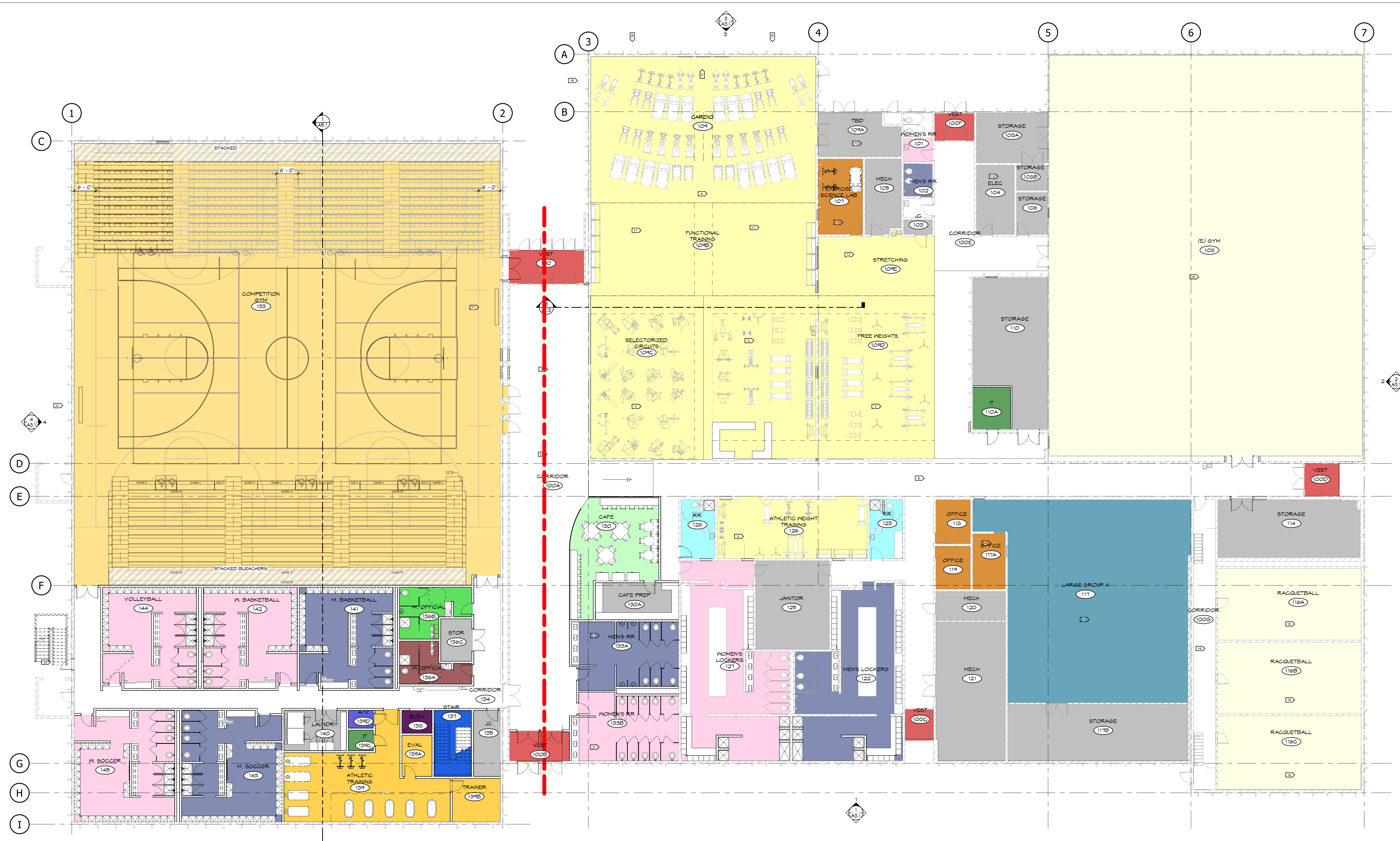
1 OVERALL NEW FLOOR PLAN A1.1 3/32" = 1'-0"
